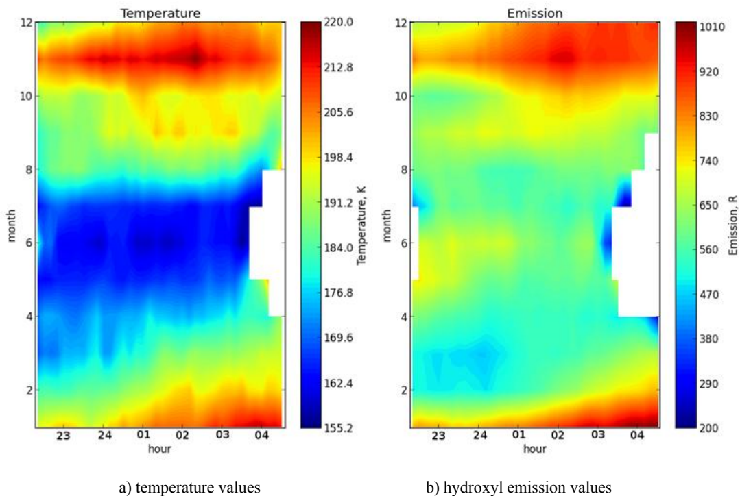
Figure 3 – The values of temperature and hydroxyl emission depending on the time of year and time of day
