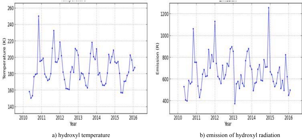
Figure 2 – Monthly average values of temperature and emission of hydroxyl radiation at an altitude of 87 km
