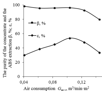
Figure 1 - Dependences of the purity of the concentrate and the ABS extraction from the air consumption at the concentration of sulphanoole 11.56 \cdot 10^{-3} \text{ kg/m}^3
