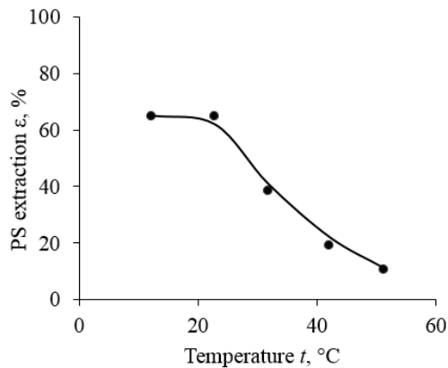
Figure 8 – Dependence of the PS extraction on the liquid temperature at the aerated liquid layer height of 0.17 m, the concentration of the mixture of surfactants of 5.41 \cdot 10^{-3} kg/m 3 and the air consumption of 0.072 m 3 /h·m 2
